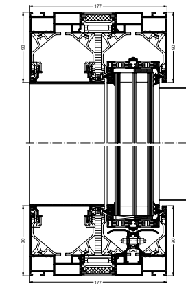
VARIANT 90/90 90/90 VERSION
