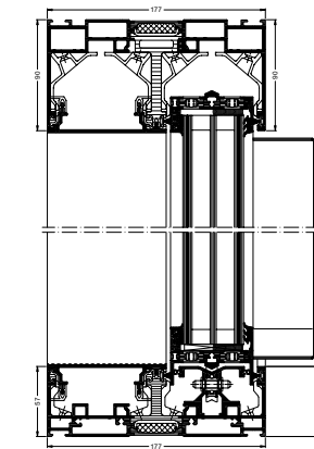
VARIANT 57/90 57/90 VERSION
